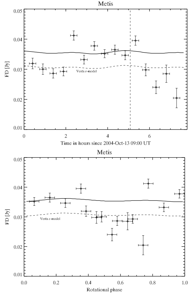
Fig. 10. Top: absolute flux prediction over time (solid line) together with the measurements (see Table 4). We used a wavelength-dependent emissivity model together with a size of 172 km and an albedo of 0.16. Bottom: the same as in the top, but now plotted against the rotational phase. The zero point in rotational phase is connected to the definition in Table 7. The dashed line indicates a model prediction with an emissivity of 0.6. This clearly shows the emissivity heterogeneity on the surface of (9) Metis. For the dashed lines we used the emissivity model for (4) Vesta.
