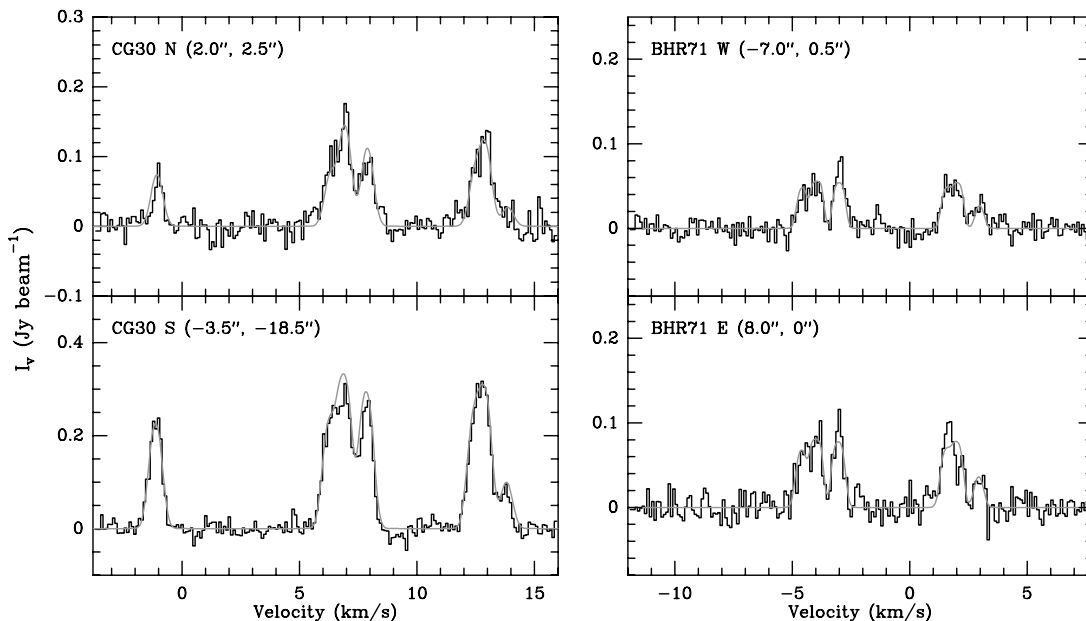
FIG. 3.— N_2H^+ spectra at the peak positions of the two cores in CG 30 (left) and BHR 71 (right). Thin dotted curves show the results of hyperfine-structure line fitting. Fit parameters are given in Table 3. [See the electronic edition of the Supplement for a color version of this figure.]
