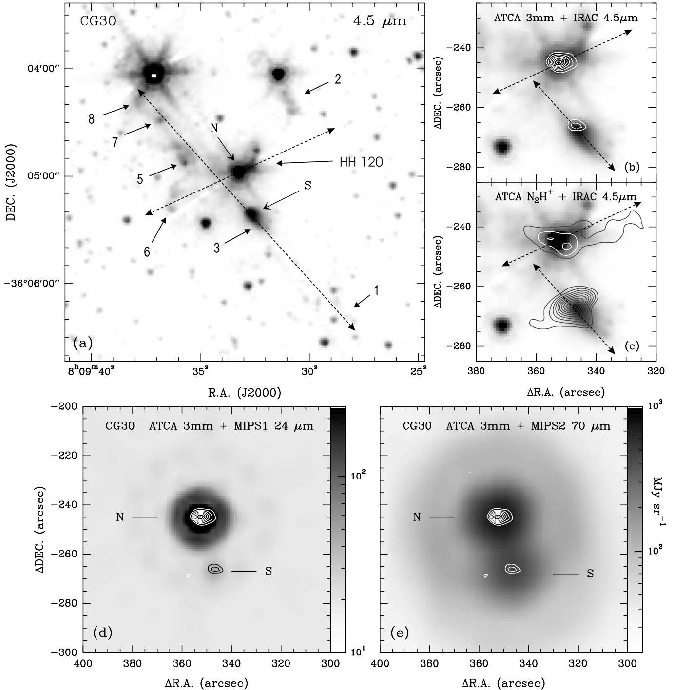
FIG. 7.— Spitzer images of CG 30. (a) Spitzer IRAC band 2 ( 4.5\ \mu\text{m} ) image of CG 30. Sources CG 30N and CG 30S are labeled as “N” and “S,” respectively. Dashed arrows show the directions of the protostellar jets. (b) IRAC band 2 image overlaid with the ATCA 3 mm dust-continuum contours (reference position at R.A. = 08^{\text{h}}09^{\text{m}}04.082^{\text{s}} , decl. = -36^{\circ}00'53.53'' , J2000.0). (c) Same, but overlaid with the ATCA \text{N}_2\text{H}^+ intensity contours. (d) Spitzer MIPS 1 ( 24\ \mu\text{m} ) image of CG 30, overlaid with the ATCA 3 mm dust-continuum contours. (e) Spitzer MIPS 2 ( 70\ \mu\text{m} ) image of CG 30, overlaid with the ATCA 3 mm dust-continuum contours.
