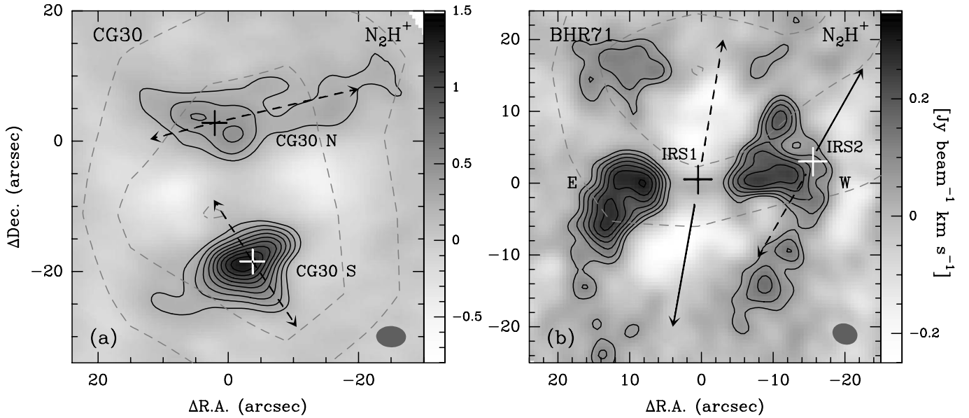
FIG. 2.—(a) Image of the N_2H^+ (1–0) intensity integrated over the seven hyperfine components for CG 30. Contours start at \sim 3\sigma ( \sigma \sim 60 mJy) with steps of \sim 2\sigma . The arrows show the directions of protostellar jets (see § 3.3). The gray dashed contours represent the 50%, 75%, and 99% levels of the N_2H^+ (1–0) emission observed with Mopra single-dish telescope (P. Barnes et al., in preparation). (b) The same for BHR 71 ( 1\sigma \sim 20 mJy). The solid and dashed arrows show the directions of the blueshifted and redshifted CO outflows (see § 3.3). The crosses in both images represent the peaks of 3 mm dust-continuum emission. Synthesized ATCA beams are shown as gray ovals.
