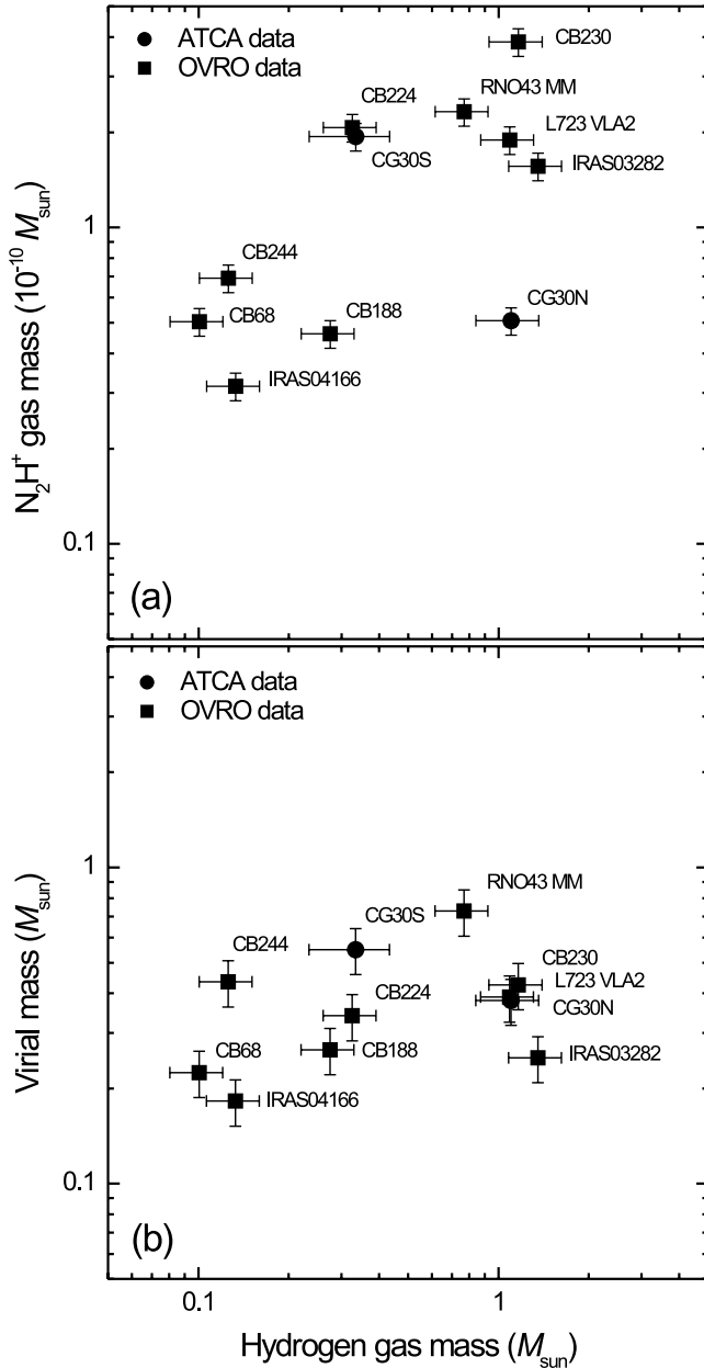
FIG. 10.—(a) N_2H^+ gas mass (derived from N_2H^+ line emission) vs. hydrogen gas mass (derived from 3 mm dust-continuum emission; the dust-continuum data of OVRO sample are taken from R. Launhardt et al. (in preparation), and (b) virial mass (derived from N_2H^+ line emission) vs. hydrogen gas mass for protostellar cores studied in Paper I and this work.
