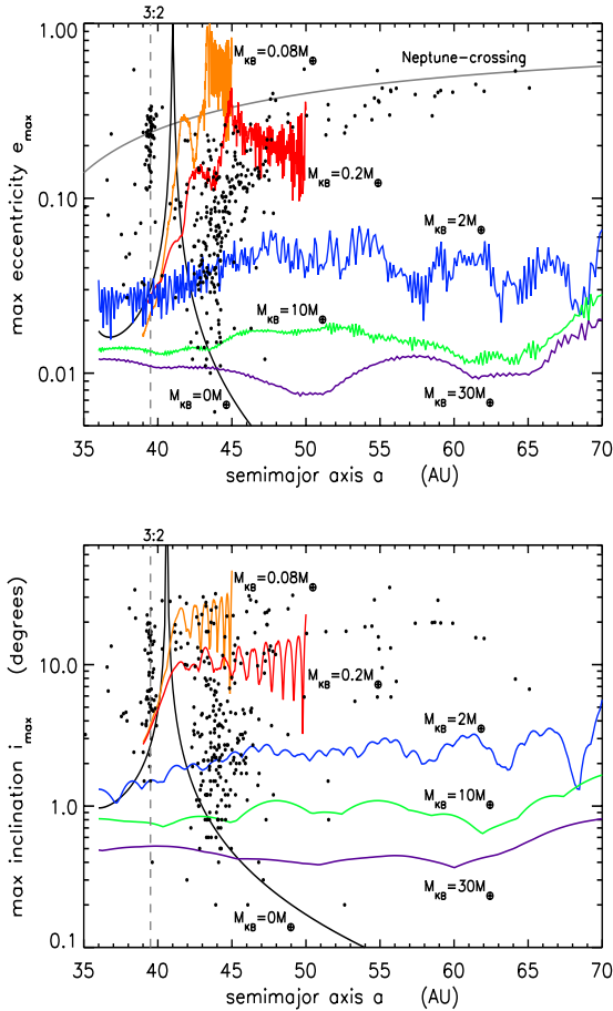
Figure 1: Dots indicate the eccentricities e and inclinations i plotted versus semimajor axes a of 373 multi-opposition KBOs reported by the Minor Planet Center. The dashed lines indicate Neptune's 3:2 resonances at 39.5 AU while the grey curve indicates the threshold for Neptune-crossing orbits. The colored curves are the maximum eccentricities e_{\max} and maximum inclinations i_{\max} achieved by various model Kuiper Belt's having a mass M_{\text{KB}} that would have been contained within the 30 < a < 50 AU interval had the model Belt extended inwards that far. In these runs the disk rings have a thickness h/a \sim 0.002 .
